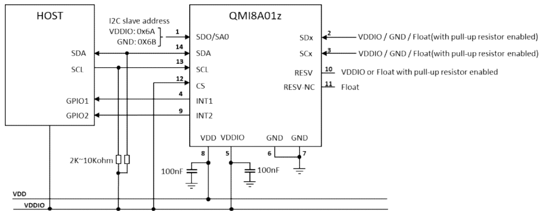
Figure 6. I3C/I2C-UI mode
