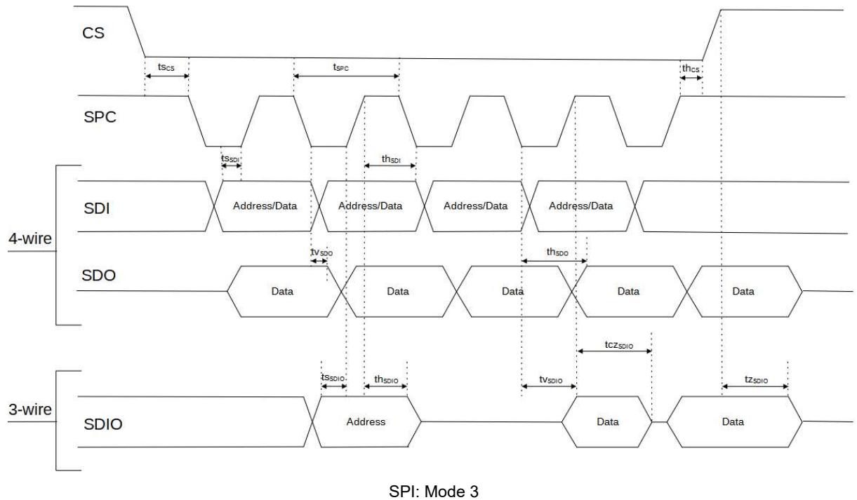
Figure 34. Timing Characteristics for SPI 3- and 4-Wire Interfaces
