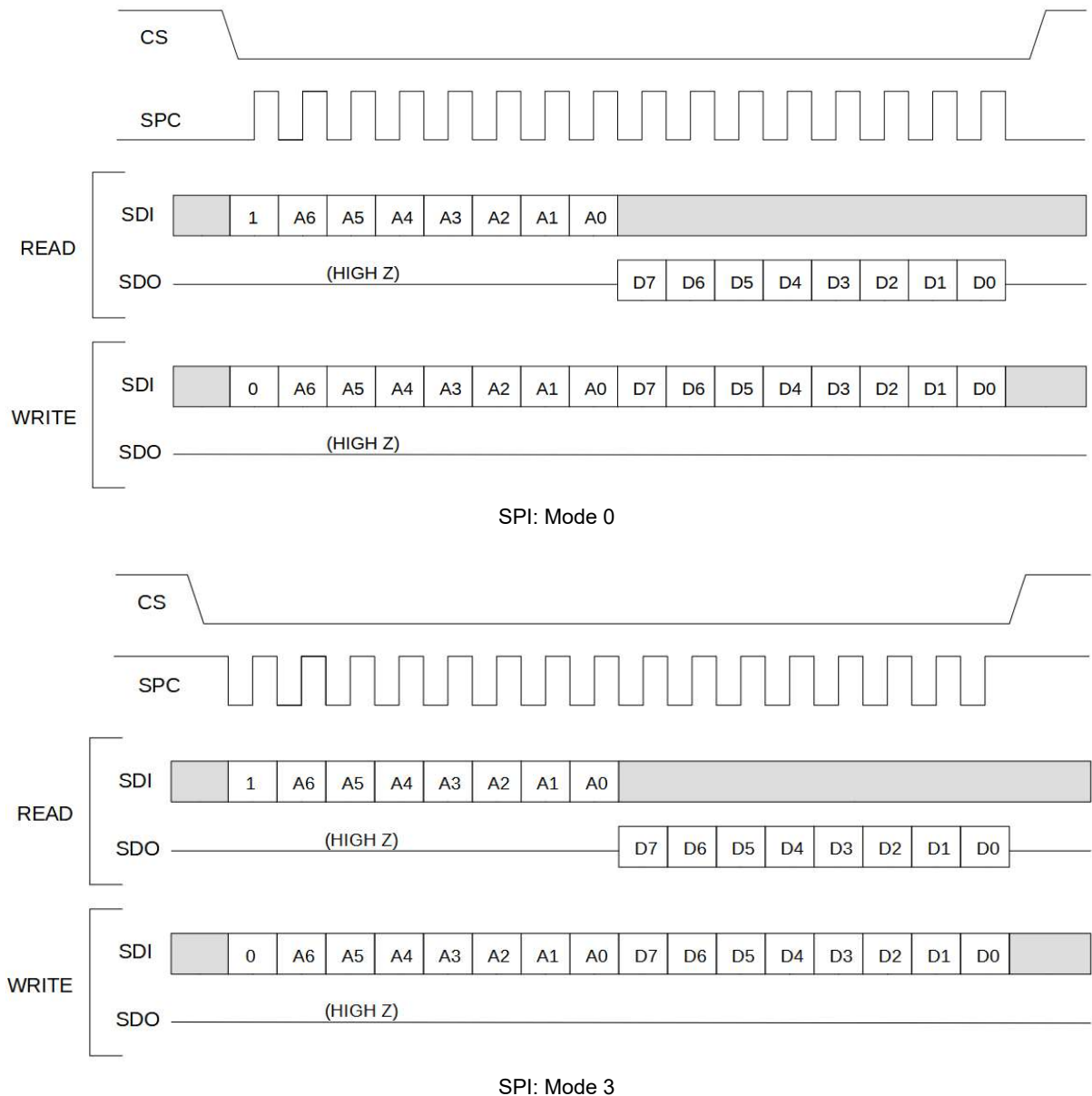
Figure 30. SPI 4-Wire Single Byte Read and Write (Mode 0 and Mode 3)
