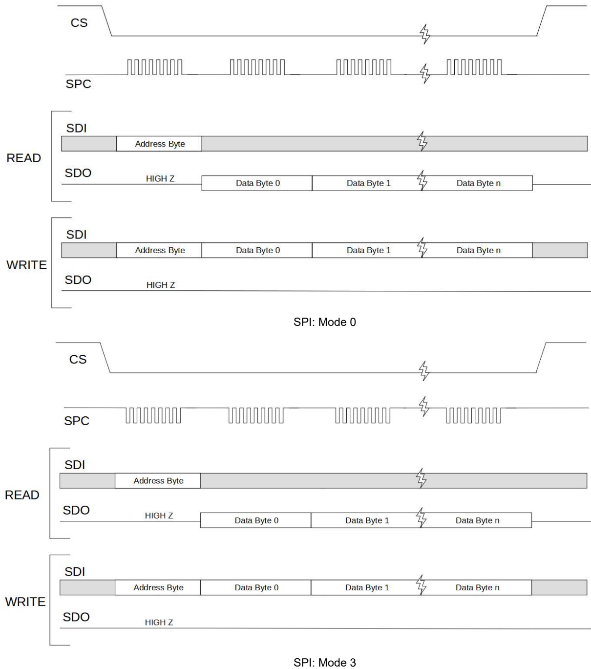
Figure 31. SPI 4-Wire Multi-Byte Read and Write Transactions
