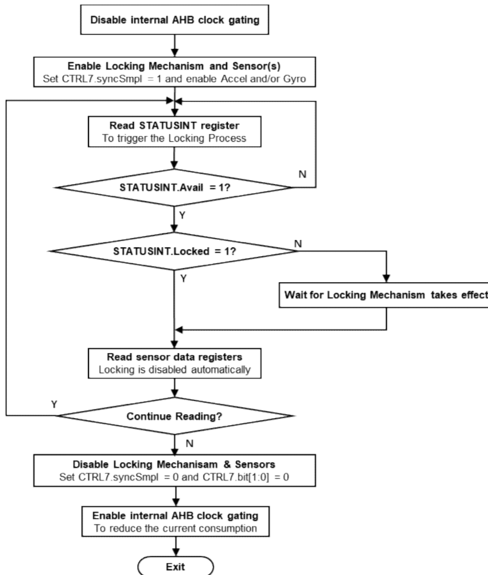
Figure 26. Data Reading Process in Locking Mechanism
