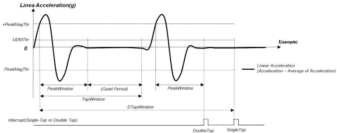
Figure 24. Tap Detect Principle
