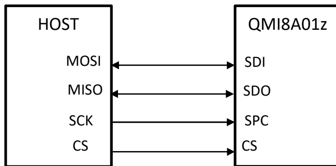
Figure 28. Typical SPI 4-Wire Connection
