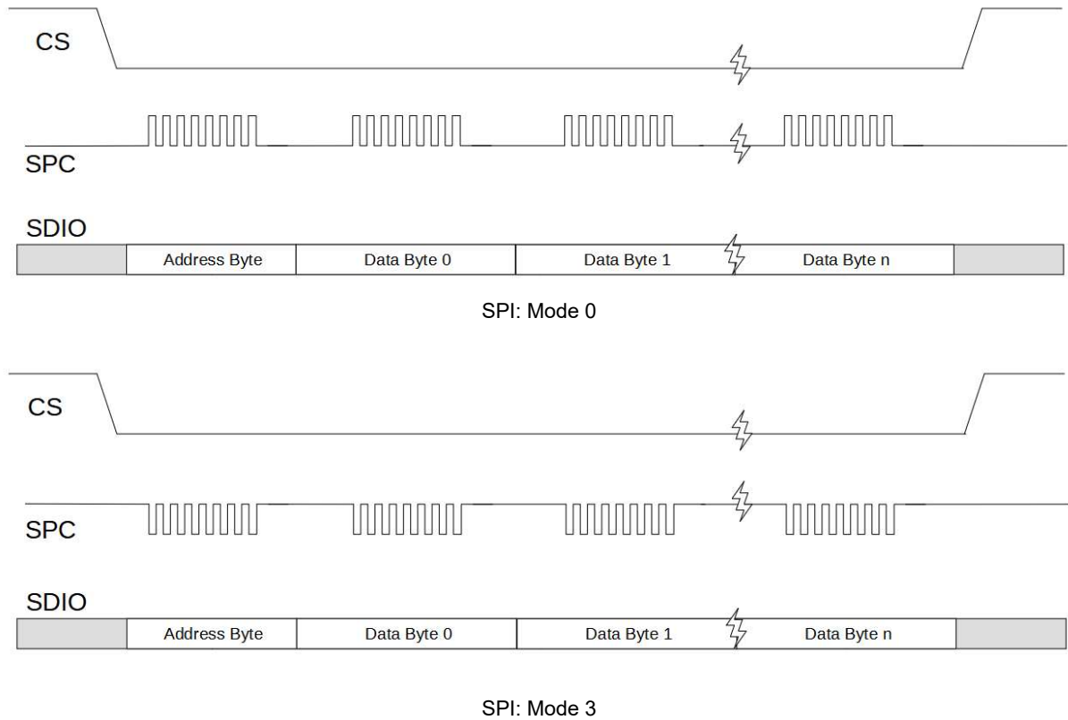
Figure 33. SPI 3-Wire Multi-Byte Read and Write Transactions
