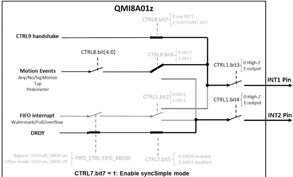
Figure 14. Interrupt Map of SyncSample Mode
