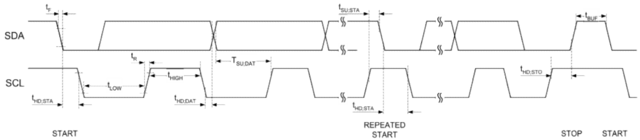
Figure 35. I2C Standard Mode Interface Timing
