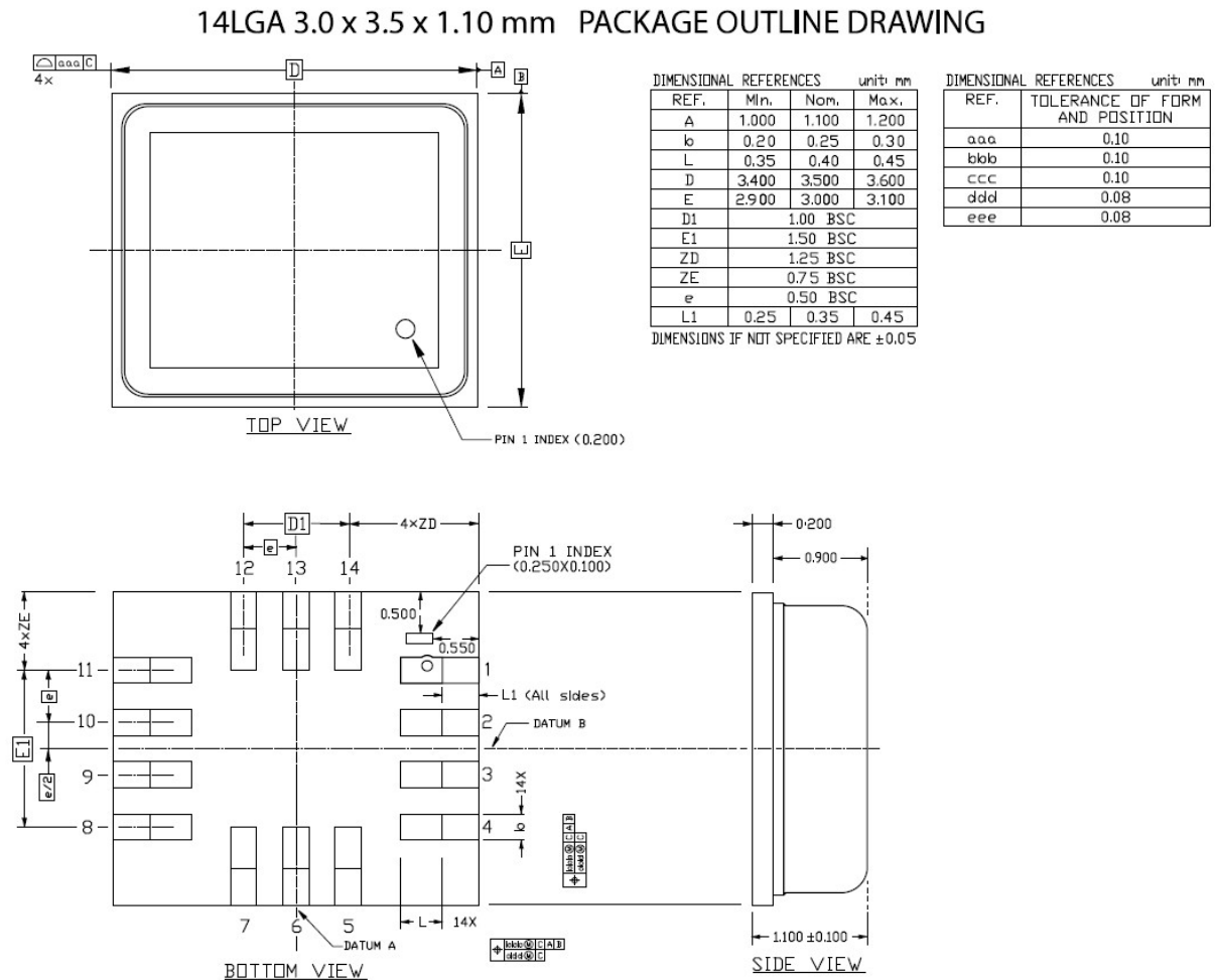
Figure 37. 14 Pin LGA 3.0 x 3.5 x 1.1 mm Package
