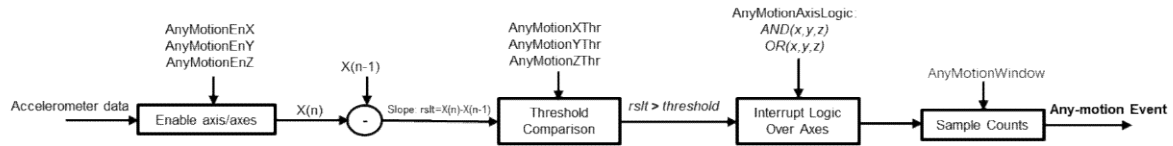
Figure 22. Any-Motion Detection Flow
