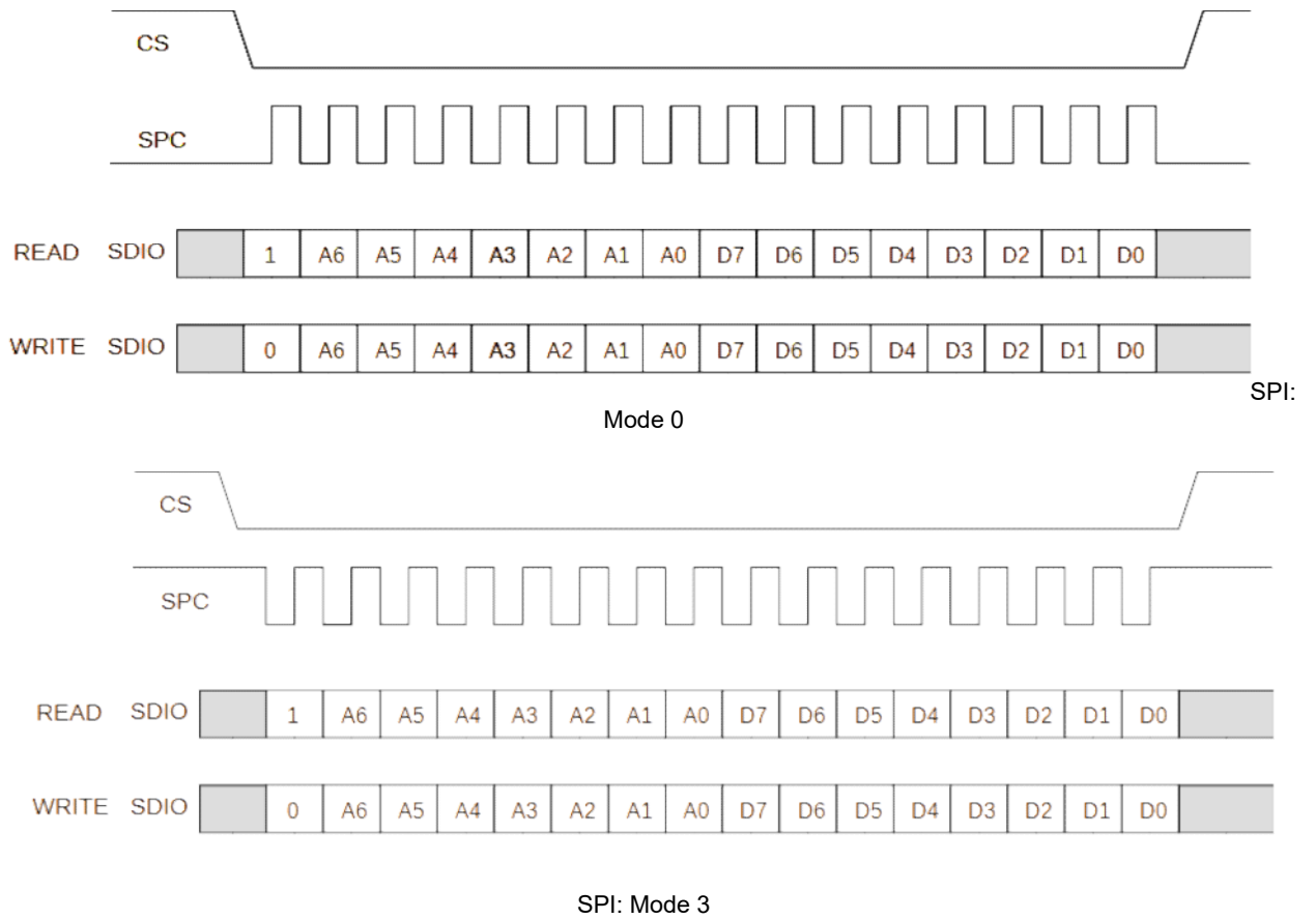
Figure 32. SPI 3-Wire Single Byte Read and Write Transactions
