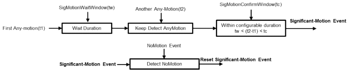
Figure 23. Significant-Motion Detection Flow
